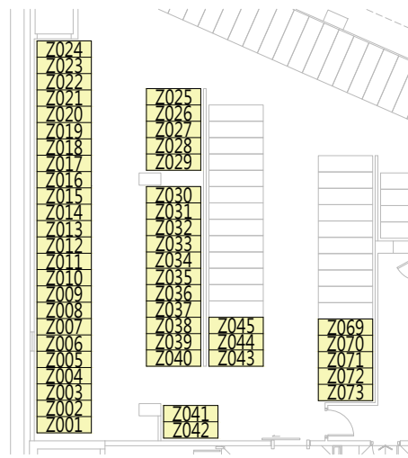
② PART PLAN OF BICYCLE PARKING SPACE 單車停車位部份平面圖
