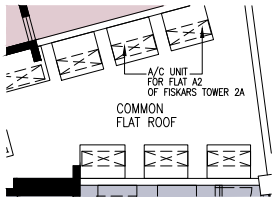
PART PLAN OF GARDEN FLOOR (2/F) OF FISKARS TOWER 2B (REFER TO AL028) FISKARS第2B座花園層(2樓) 部分平面圖 (參閱AL028)
