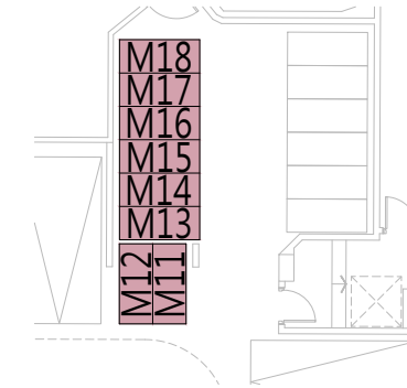
① PART PLAN OF RESIDENTIAL MOTOR CYCLE PARKING SPACE 住宅電單車停車位部份平面圖
